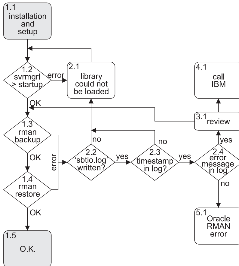
Figure 22. Problem isolation for RMAN
