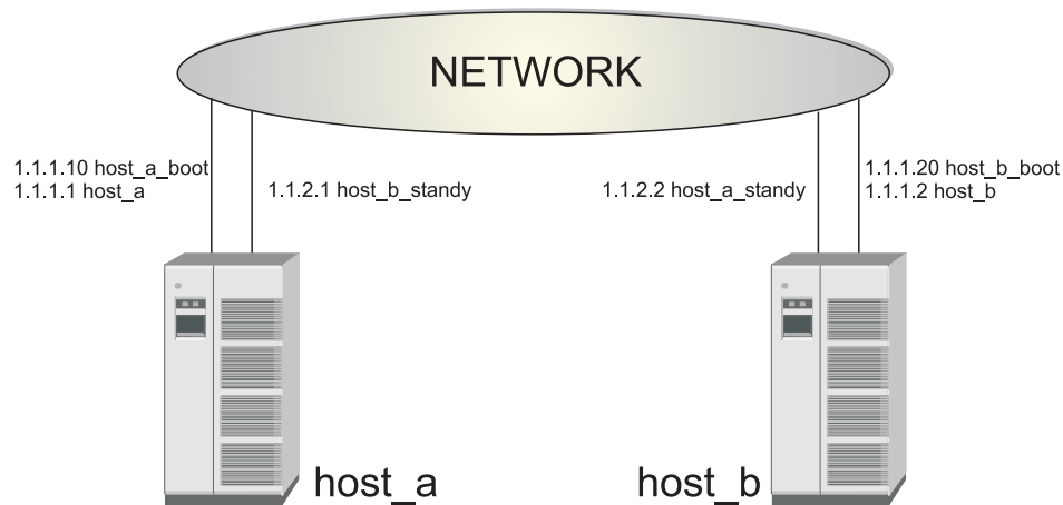
Figure 5. Sample environment for HACMP takeover
