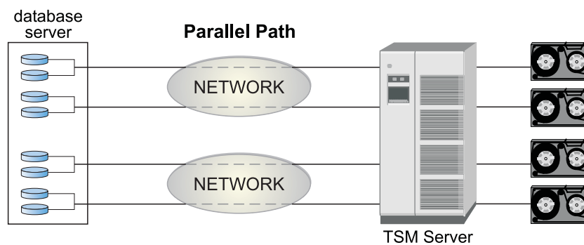
Figure 19. Parallel (multiple) paths
