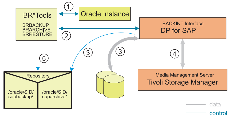
Figure 3. Data Protection for SAP with BR*Tools by using the BACKINT Interface
